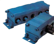
Flow Dividers
