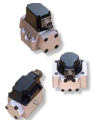
Servo Valves
